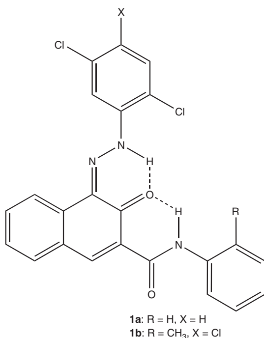
Figure 2 Azonaphtharylamine pigments ( 1 ) derived from dichloro- or trichloroanilines as diazo components
