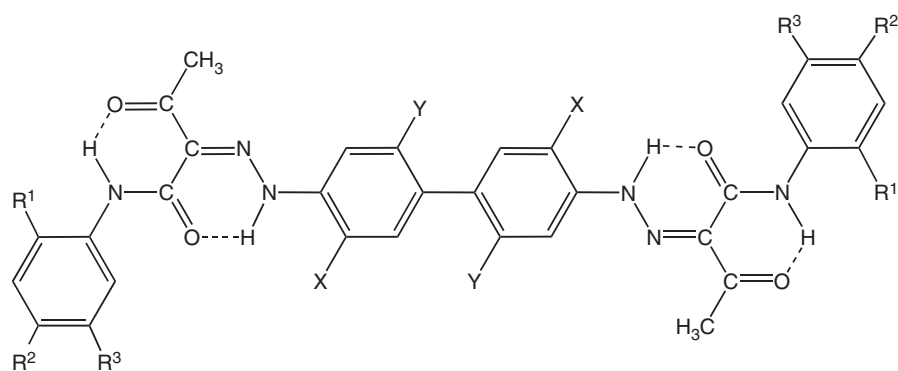
Figure 3 The general structure of a diarylide yellow pigment ( 2 )
