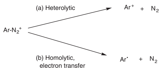
Scheme 2 General mechanisms of dediazotiation
